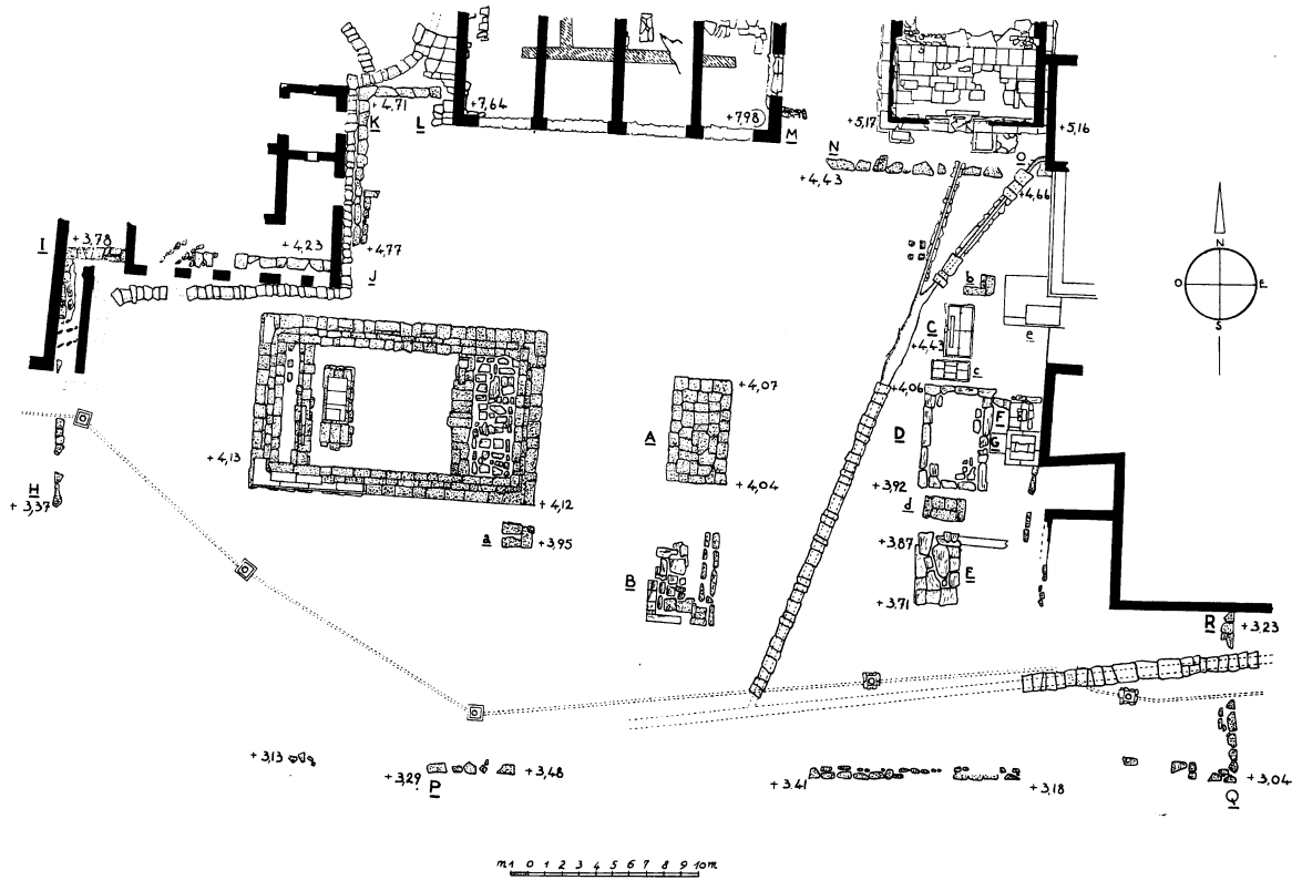
Plate 8.17. The Sanctuary of the Twelve Gods (the Dodekatheon) at Delos.
