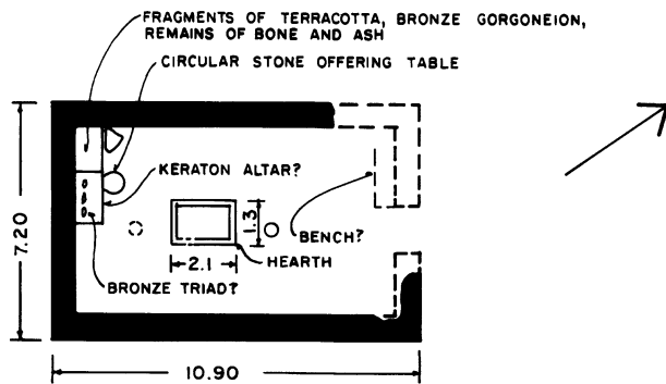
Dreros - 8th century B.C.
