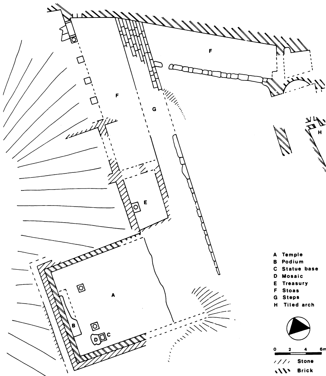
Plate 8.16. The Sanctuary of Asklepios at Lebena.
