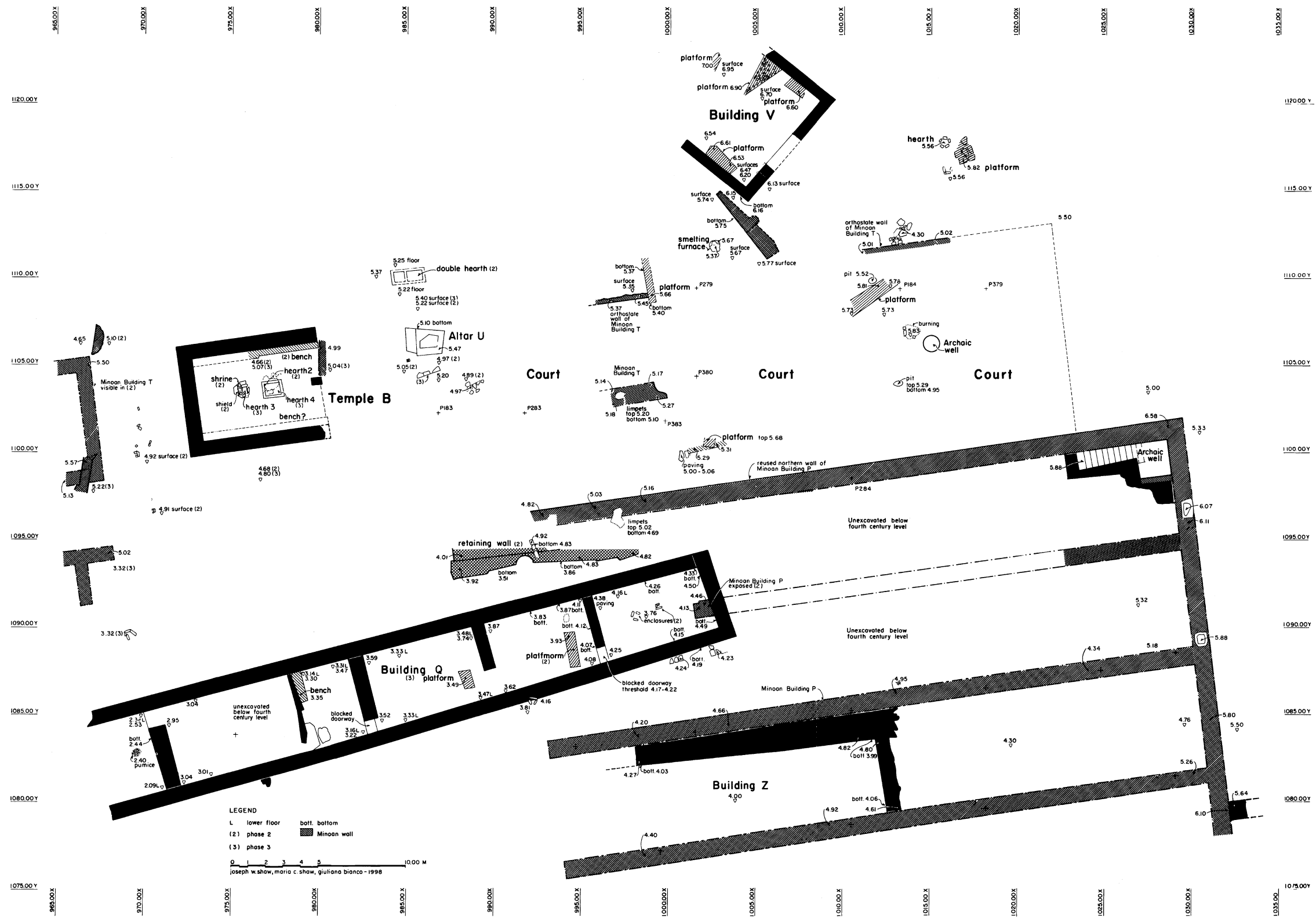
Foldout F. Greek Sanctuary, features in the area during the time of Temple B, Phases 2 and 3. Scale 1:250.
